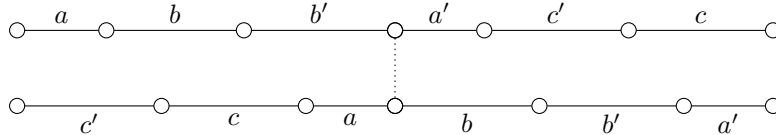
Figure 6.2: Interval exchange corresponding to the orientation covering.
