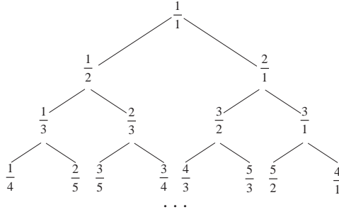
Figure 4 The Stern-Brocot tree
