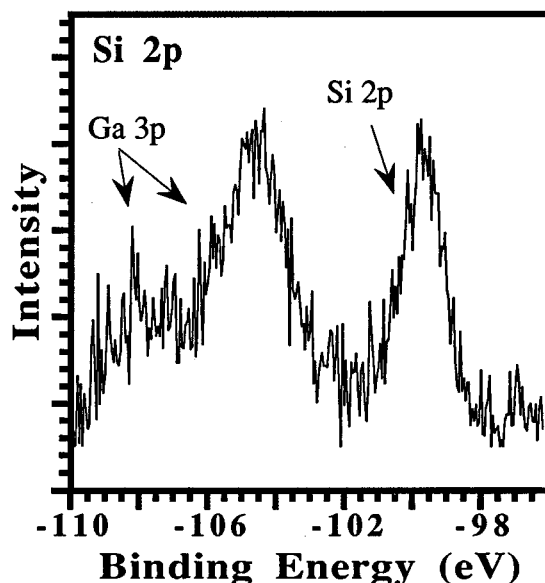
FIG. 2. Si 2p XPS spectrum from a sample irradiated with 3000 laser pulses at 25\text{ mJ/cm}^2 in a WF_6/SiH_4/H_2/Ar gas mixture.
