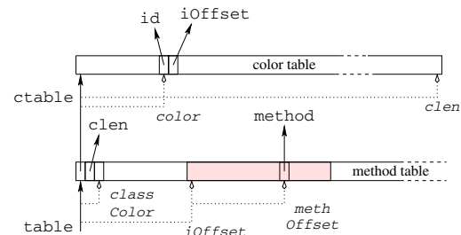
The preamble is common to both mechanisms. The implementation resembles PH, apart from the fact that the interface position results from a load instead of being the result of specific hashing. The location of the color can be the method table of the target class that is not represented here. The loads concern different memory areas and they can yield 3 cache misses. Moreover, the recomputable color table requires an extra indirection, together with its size ( clen ) and bound checking for subtype testing, and the color itself requires memory access (not represented in the diagram).
