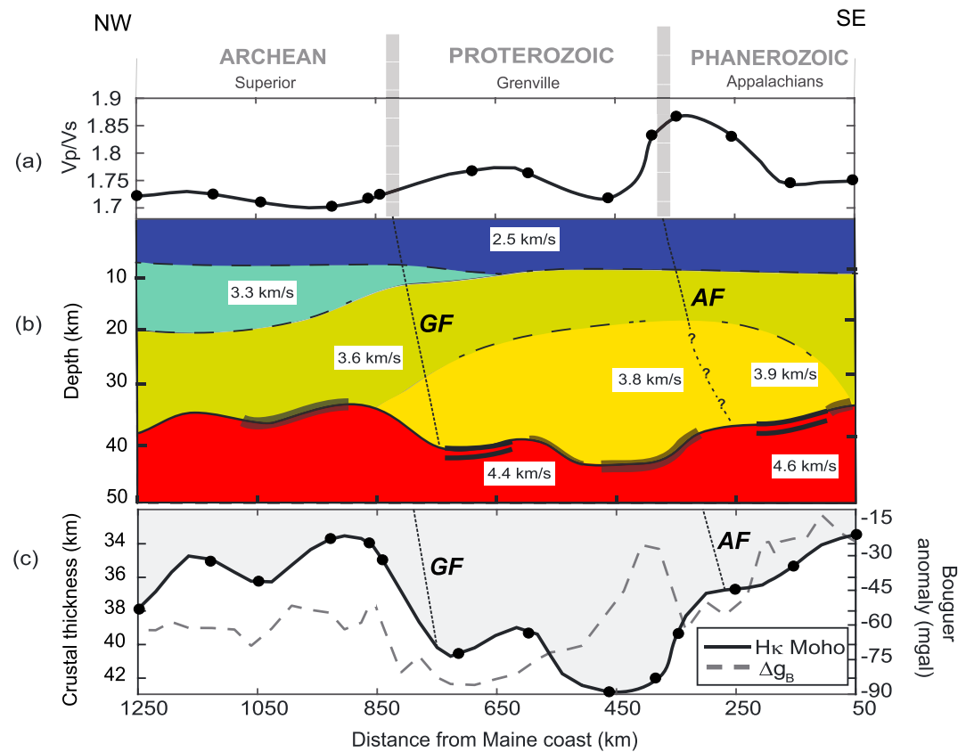
Figure 8. Structure along the QM-III NW-SE profile, based on receiver function modeling. (a) V_p/V_s ratios from H-k stacking. (b) Shear wave velocity profile based on Bayesian inversion, interpolated between individual stations. Thick semitransparent lines indicate regions with a gradational Moho; double lines indicate a doubled Moho discontinuity. (c) Crustal thickness and Bouguer gravity anomaly. GF: Grenville Front and AF: Appalachian Front.
