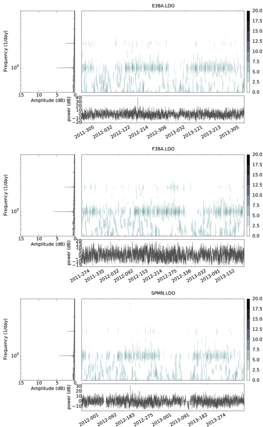
Figure 9. Time–frequency representation of power at 100 s for the barometric pressure recorded at TA stations E38A, F38A, and SPMN during the 2.5-year window in Figure 8. Again, 24- and 12-hr periodic components are present during the summer and absent in the winter. During the summer, power is high during local daylight hours and low in the night. The color version of this figure is available only in the electronic edition.
