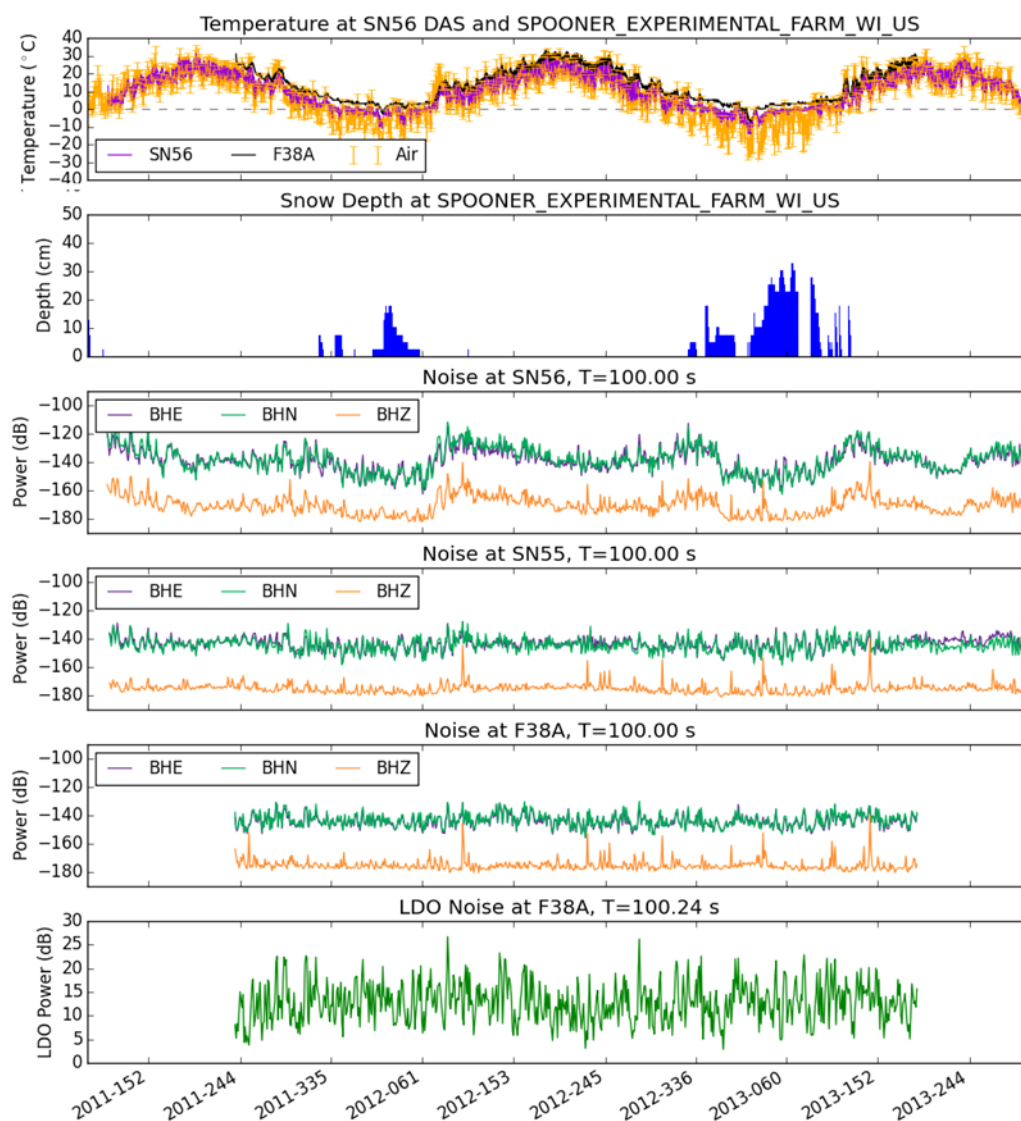
Figure 11. Noise at 100 s decreases at SN56 during the winter, while the ground is frozen and covered with snow. Compared with SN56, horizontal long-period noise at SN55 does not change much throughout the year. Minimum and maximum daily air temperatures from a nearby GHCN climate station (Menne et al. , 2012) and hourly temperatures recorded by the DAS at SN56 and F38A are shown. (DAS temperature at SN55, not shown, is within 1°–2°C of SN56.) The daily mean power at 100 s on BHZ, BHN, and BHE channels is plotted for SN56 and nearby TA station F38A. Daily mean power at 100 s is also shown for the atmospheric pressure at F38A. The color version of this figure is available only in the electronic edition.
