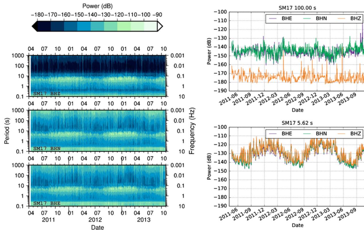
Figure 4. Daily average PSDs at station SM17 for 2.5 years, including slices at 5 and 100 s. A possible horizontal-to-vertical resonance peak is visible between 0.25 and 0.3 s (3–4 Hz). The color version of this figure is available only in the electronic edition.
