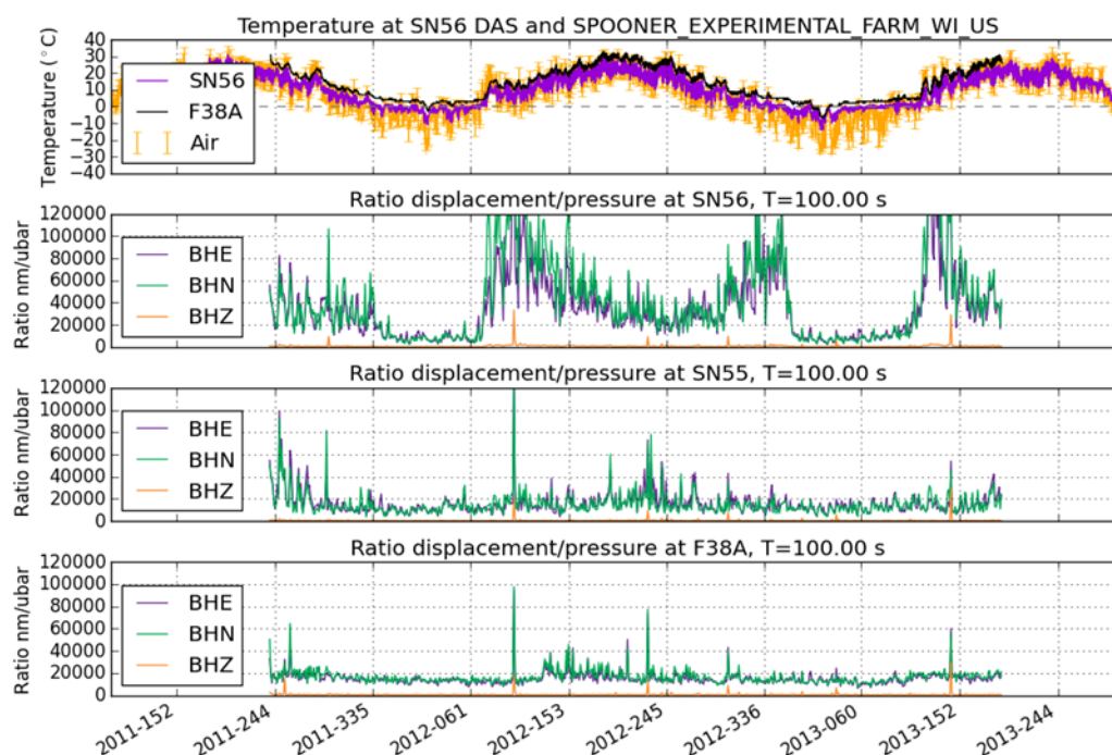
Figure 15. Daily ratio of displacement-to-pressure spectral amplitudes for SN56, SN55, and F38A. (Because SPREE stations did not record atmospheric pressure, the daily displacement spectra of SN56 and SN55 were divided by the daily pressure spectra from F38A.) The displacement-to-pressure ratio at F38A and SN55 remains relatively steady year-round. SN56 shows large displacement-to-pressure ratios in spring and fall that cannot be explained by local ground tilts alone. These large amplitudes coincide with freezing and thawing, as shown by the DAS and air temperatures. The color version of this figure is available only in the electronic edition.
