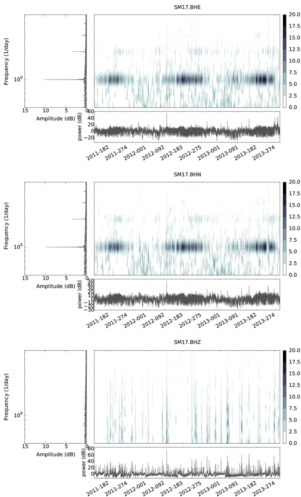
Figure 8. Time–frequency representation of power at 100 s at SPREE station SM17 for 2.5 years. Horizontal components show clear spectral peaks at periods of 24, 12, 8, and 6 hrs (1, 2, 3, and 4 cycles/day). Energy at these periods is strong during summer and decreases during winter. These peaks are absent on the vertical component. The color version of this figure is available only in the electronic edition.
