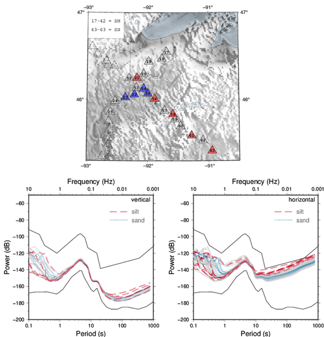
Figure 10. Lifetime average power spectra for SPREE stations SM17-25 and SN52-63. Stations in fine-grained, organic-rich material (SM21, SN56, SN58, SN61, SN63) have higher average horizontal long-period noise levels than their neighbors. In contrast, the four stations in the Grayling sand unit (SM22, SM23, SN54, and SN55) are some of the quietest stations and differ by only a few decibels at long periods on the horizontal components. The color version of this figure is available only in the electronic edition.
