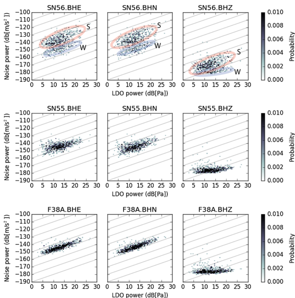
Figure 14. Daily mean noise versus daily mean atmospheric pressure noise (LDO, recorded at F38A). Noise on the horizontal components of SN56, SN55, and F38A all show a linear relationship with atmospheric pressure noise. Diagonal lines indicate a slope of 1. For SN56, the circled areas labeled W indicate values that occur during winter (December–March); values in circled areas labeled S occur during the rest of the year. The color version of this figure is available only in the electronic edition.
