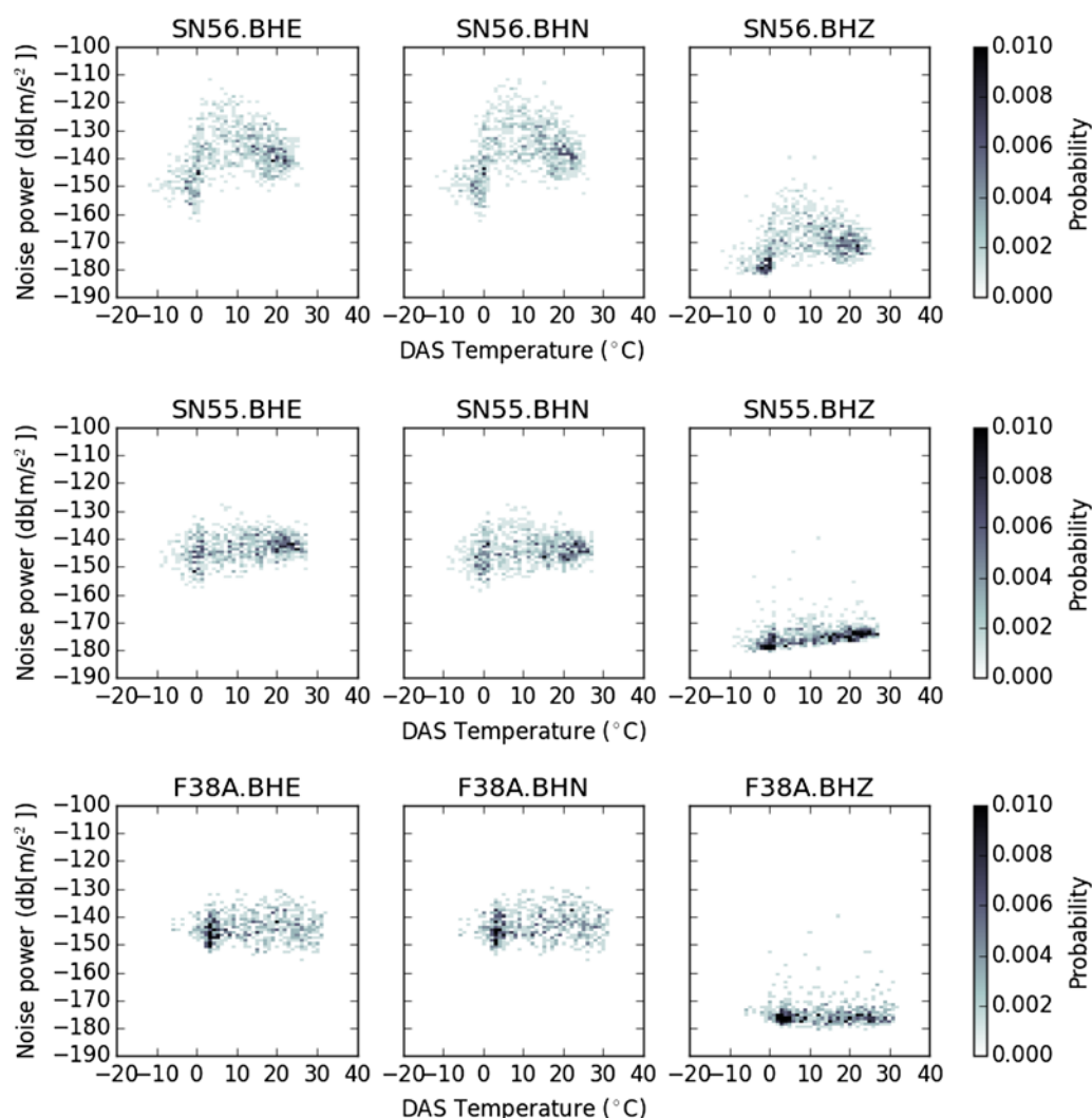
Figure 12. Daily mean noise versus daily mean temperature at SN56, SN55, and F38A. SN56 is noisiest at temperatures between 0°C and 10°C and quietest below 0°C. Noise at SN55 increases slightly with temperature; this is clearest on the vertical component. Noise at F38A does not vary with temperature. The color version of this figure is available only in the electronic edition.
