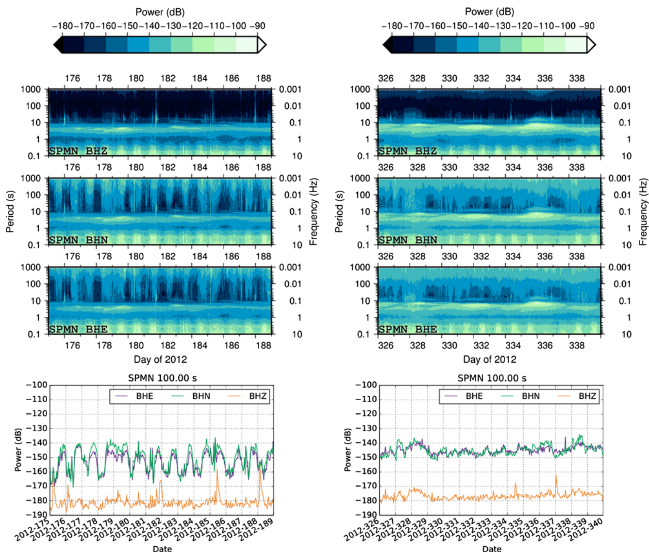
Figure 7. Power at TA station SPMN for 14 days in (left) summer and (right) winter, including slices at a period of 100 s. Ticks are at midnight UTC; local time is UTC – 5 during summer and UTC – 6 during winter. The color version of this figure is available only in the electronic edition.
