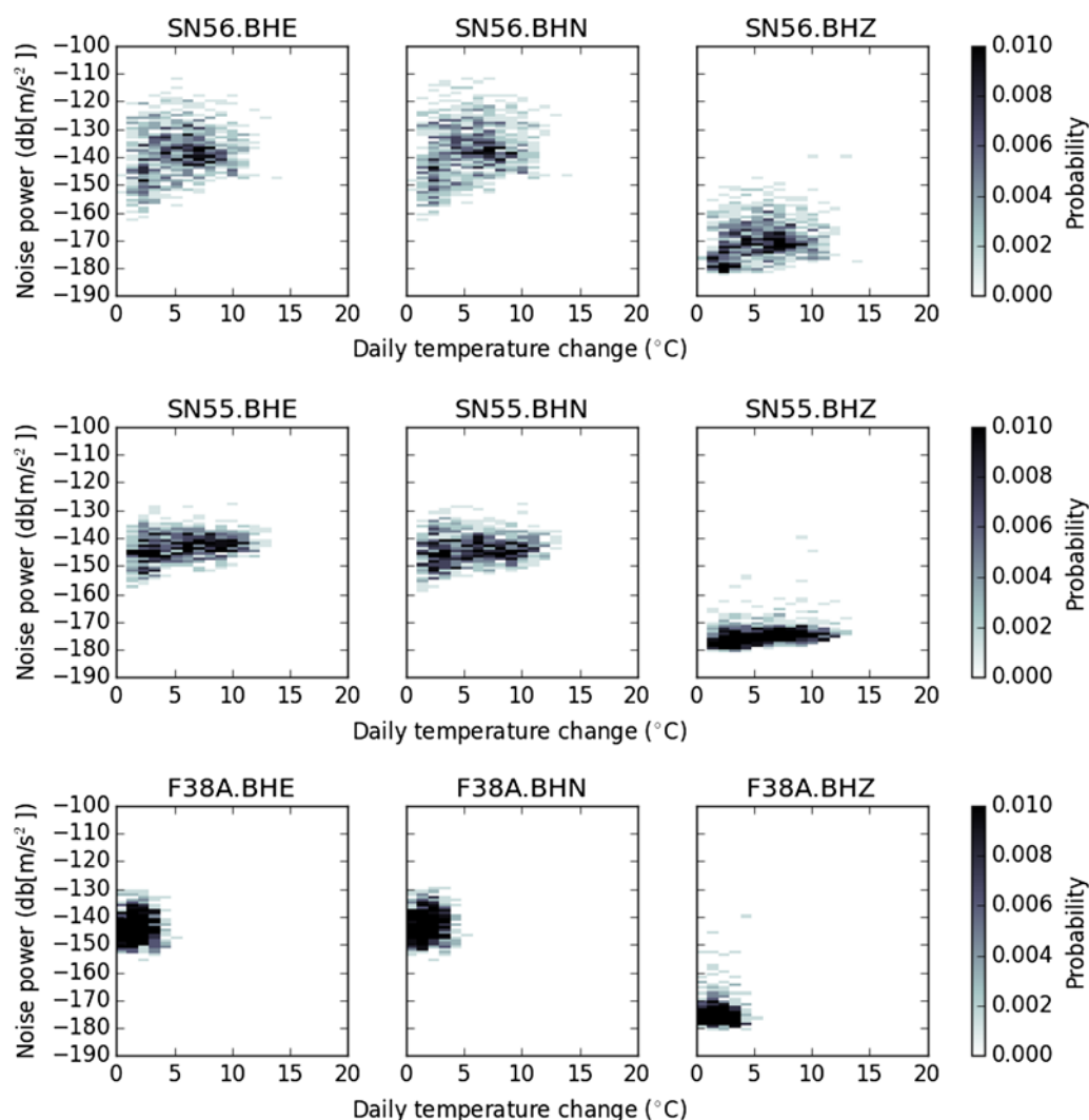
Figure 13. Daily mean noise versus daily temperature change at SN56, SN55, and F38A. Noise at SN56 appears to depend somewhat on the daily temperature change. At SN55, temperature changes appear to have a smaller effect on noise levels. At F38A, the vault temperature is more stable than at the SPREE stations and appears to have little effect on noise levels. The color version of this figure is available only in the electronic edition.
