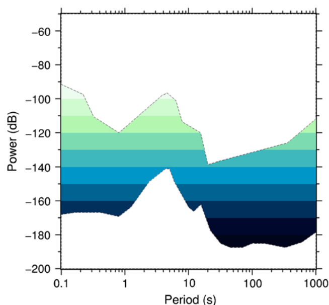
Figure 2. Peterson new high- and low-noise models. Intermediate values are filled using the same scale as Figures 3, 4, and 5. The color version of this figure is available only in the electronic edition.
