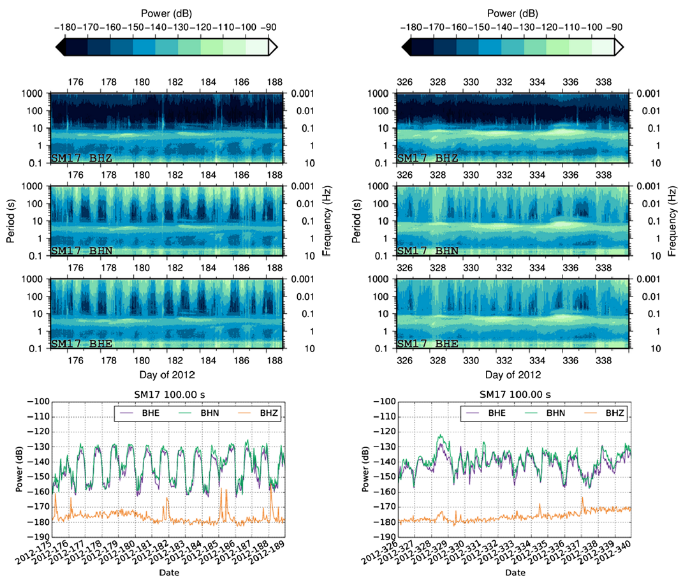
Figure 6. Power at SPREE station SM17 for 14 days in (left) summer and (right) winter, including slices at a period of 100 s. Ticks are at midnight UTC; local time is UTC – 5 during summer and UTC – 6 during winter. The color version of this figure is available only in the electronic edition.
