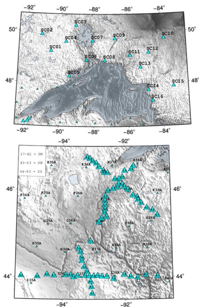
Figure 1. Topographic map of Superior Province Rifting Earthscope Experiment (SPREE) and nearby Transportable Array (TA) stations. Stations SC01–SC16 expand TA-style spacing north of Lake Superior. SM17–SM42 follow the center of the Midcontinent Rift’s Bouguer gravity anomaly. The northern line (SN43–SN63) crosses the anomaly at its widest point, and the southern line (SS64–SS83) crosses it at its narrowest point. The color version of this figure is available only in the electronic edition.
